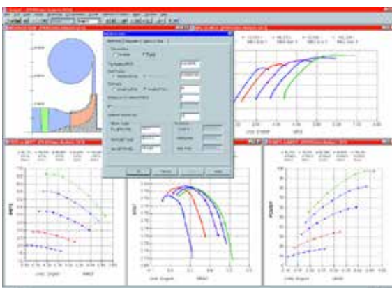
Multiple speed line performance map with IGV and volute.
